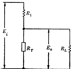
FIG. 4-74.—Nonlinear resistance regulator.
